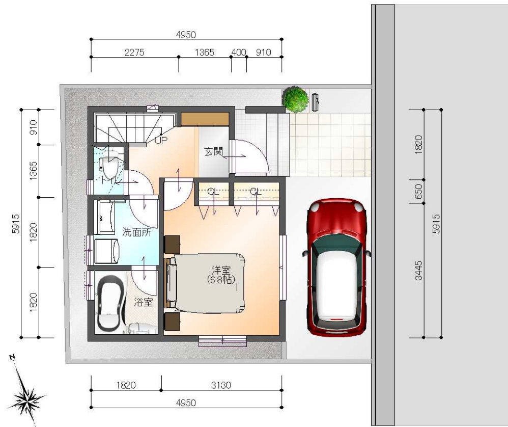
1st Floor
